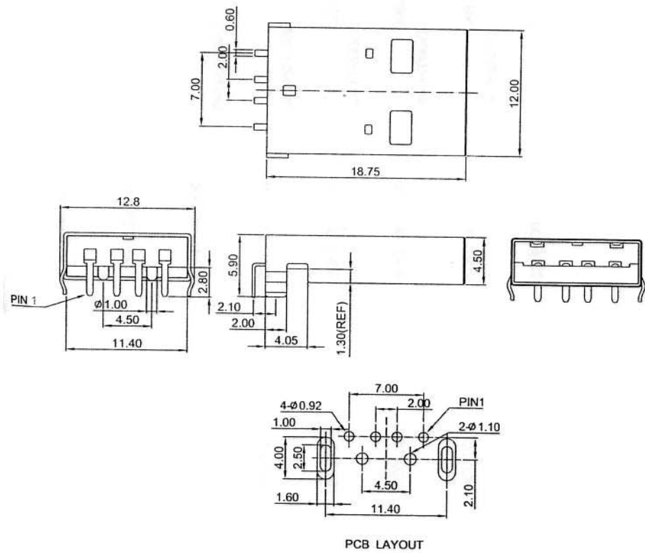
PCB LAYOUT
