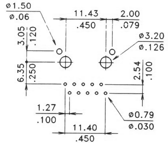
PC Board Layout (FOR 10P10C)
