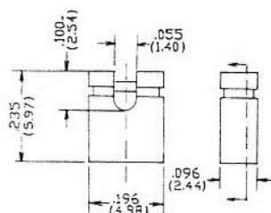
MINI JUMPER PITCH=2.54MM OPEN END MJ 3611O
