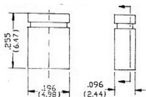
MINI JUMPER PITCH=2.54MM CLOSE END MJ 3611C
